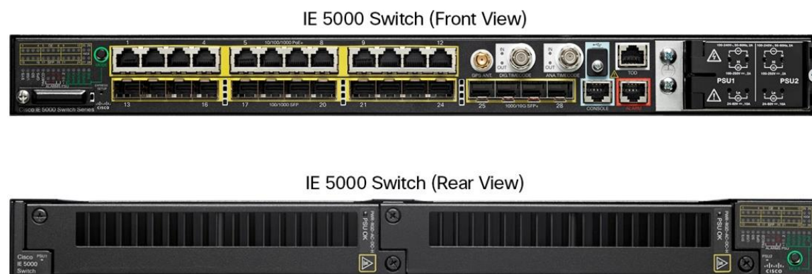
Figure 1. IE 5000 switch
